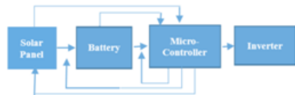
Fig. 2: Block Diagram of circuit
